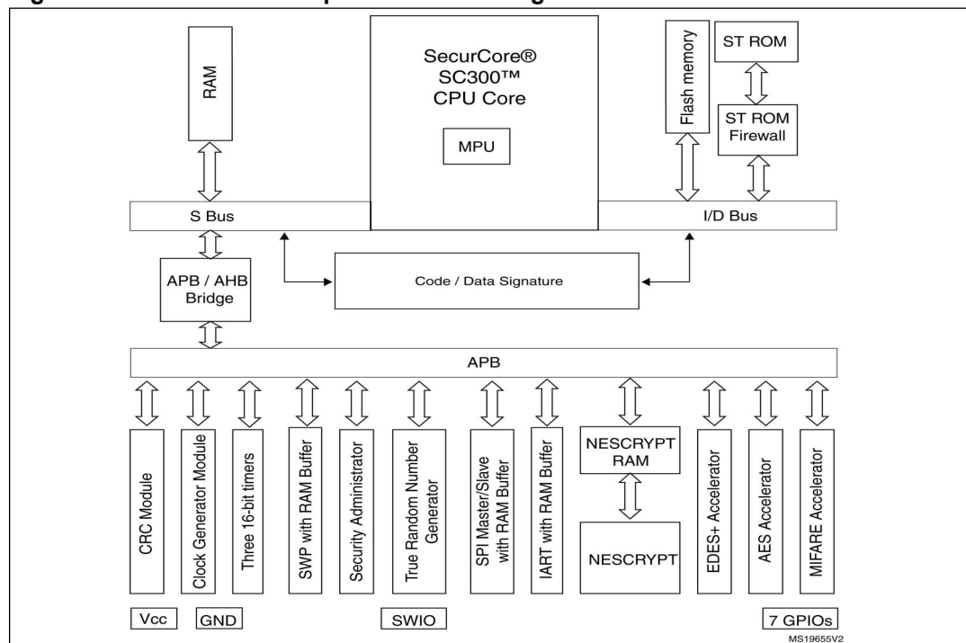
Figure 1. ST33G1M2 E02 platform block diagram
