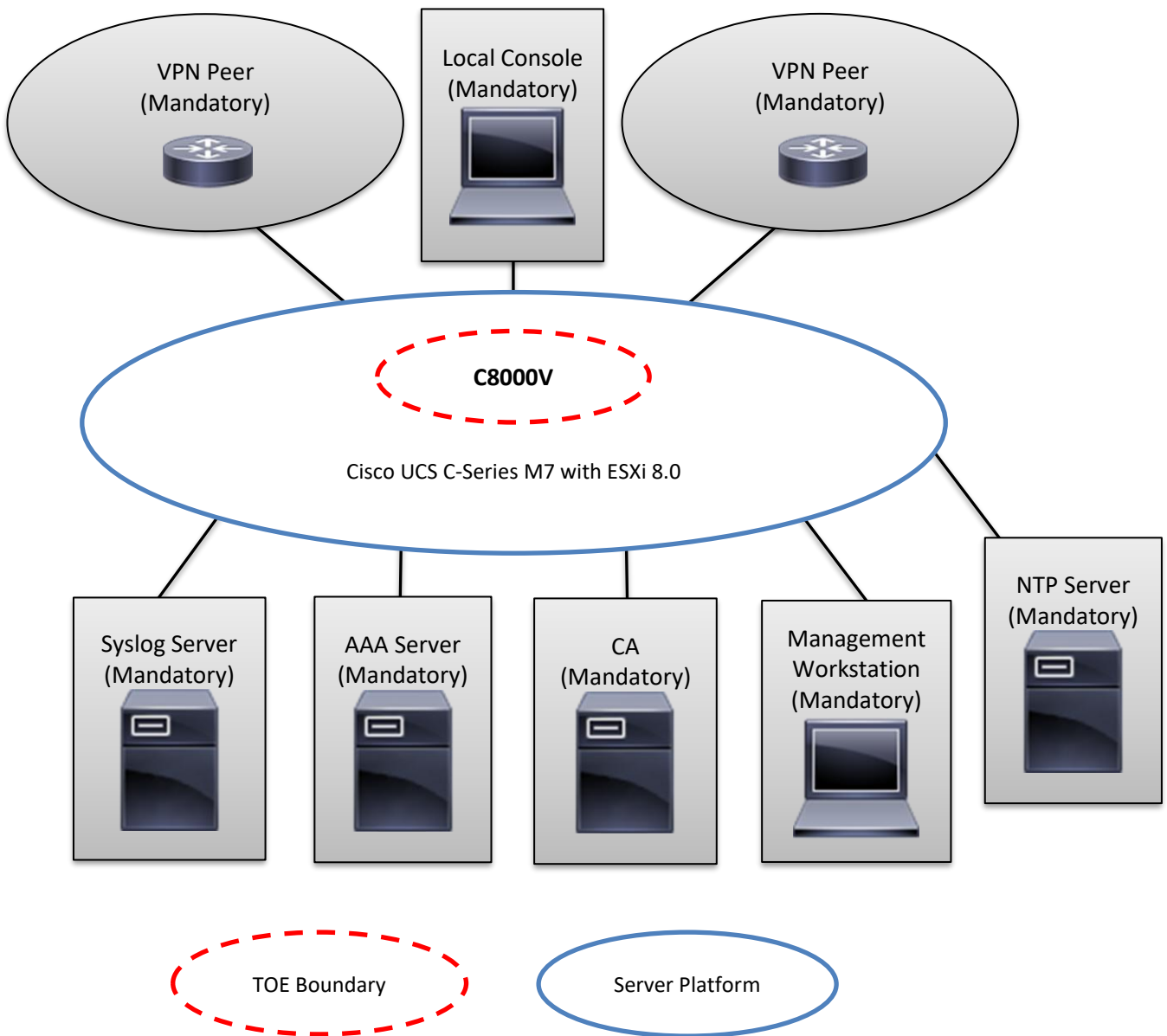
Figure 1 Example Deployment for C8000V
