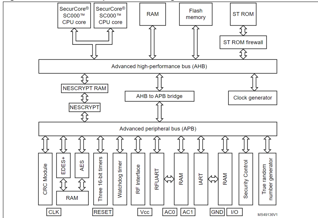
Figure 1. ST31P450 A08 platform block diagram
