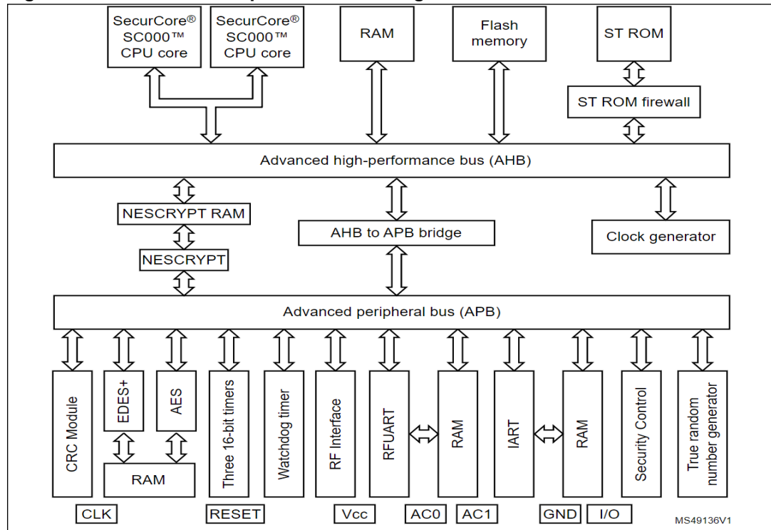
Figure 1. ST31P450 C03 platform block diagram
