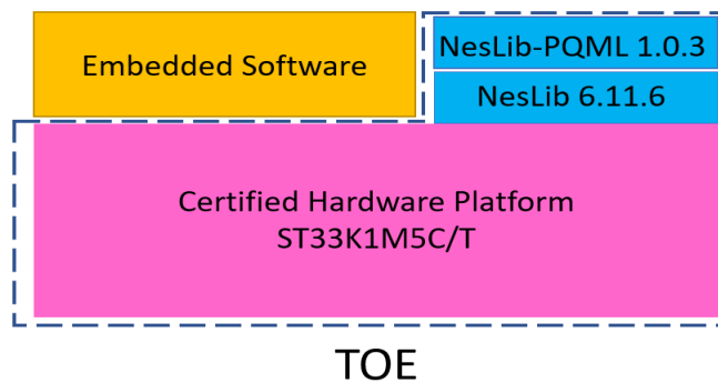
Figure 1. TOE overview
