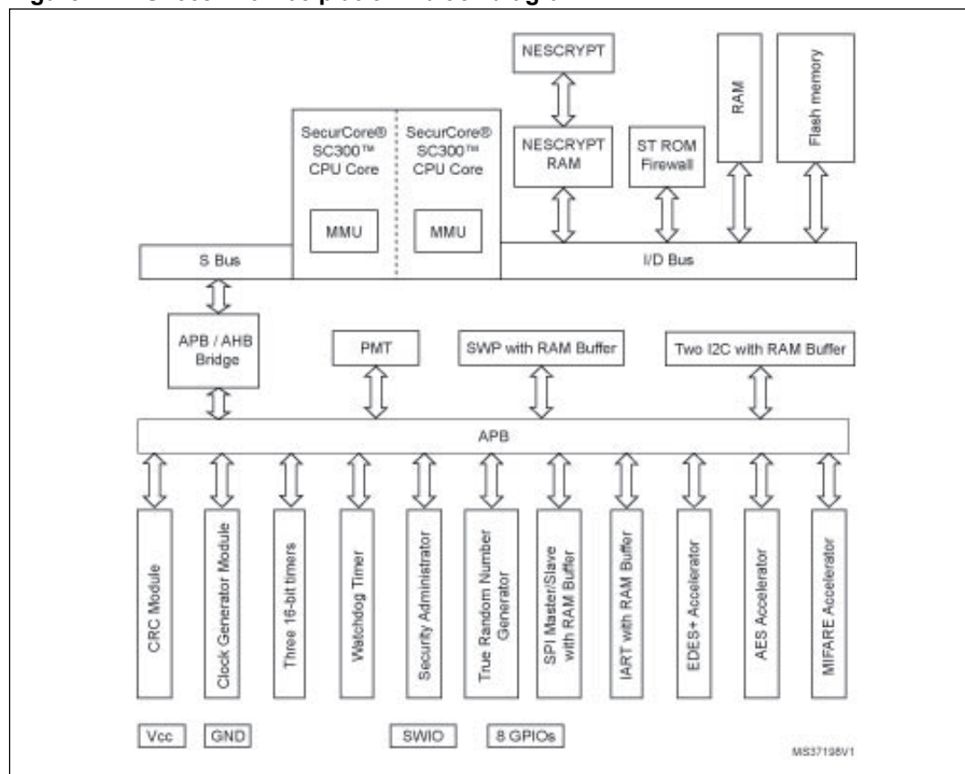
Figure 1. ST33J2M0 C05 platform block diagram
