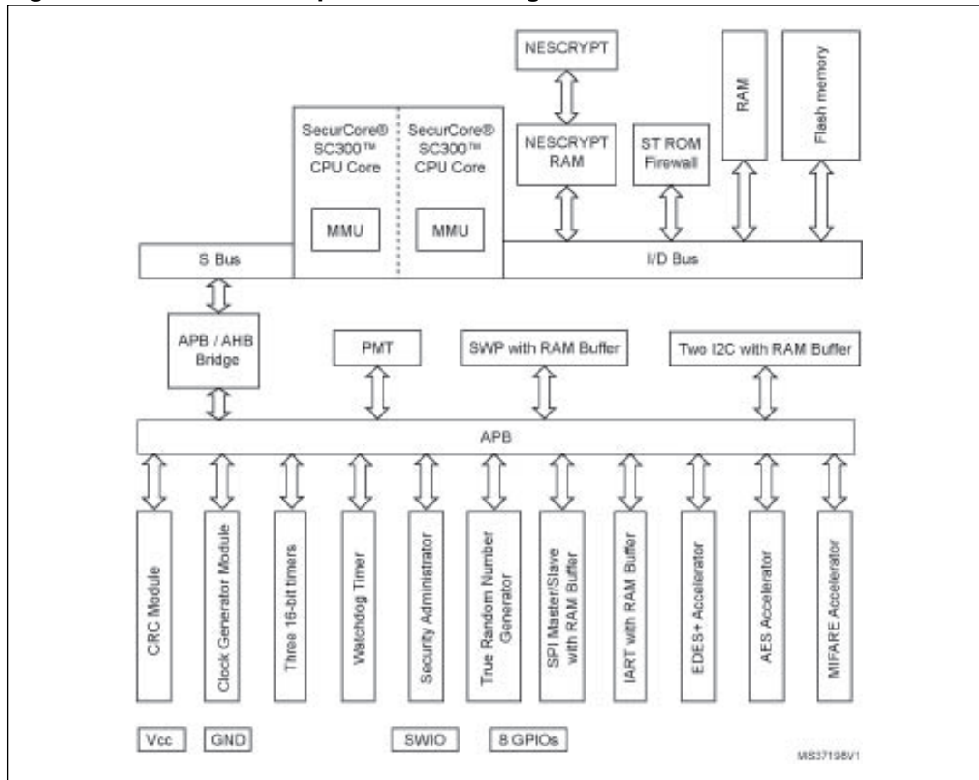
Figure 1. ST33J2M0 F03 platform block diagram
