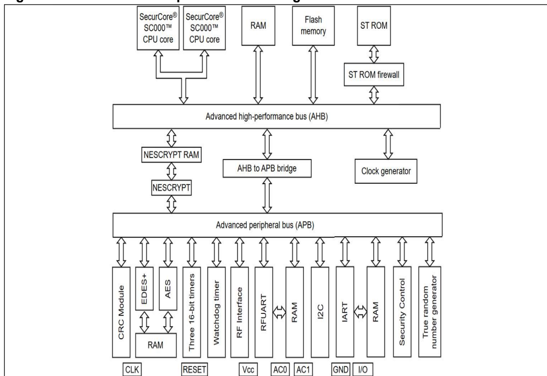
Figure 1. ST31R480 A02 platform block diagram
