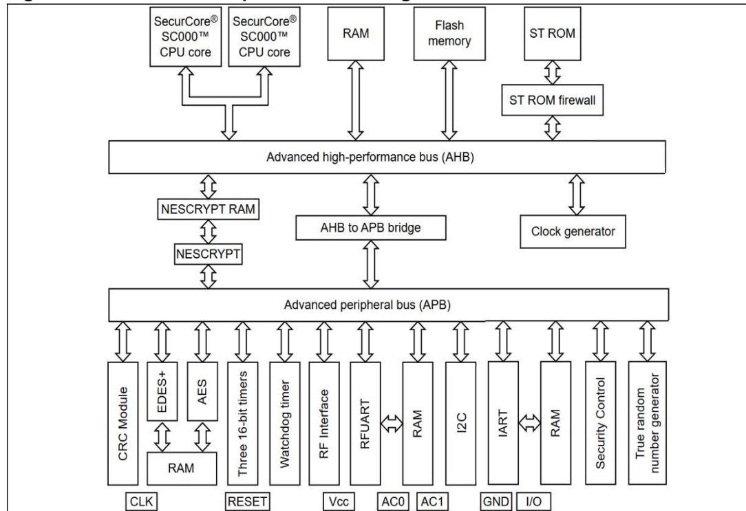
Figure 1. ST31R480 C02 platform block diagram
