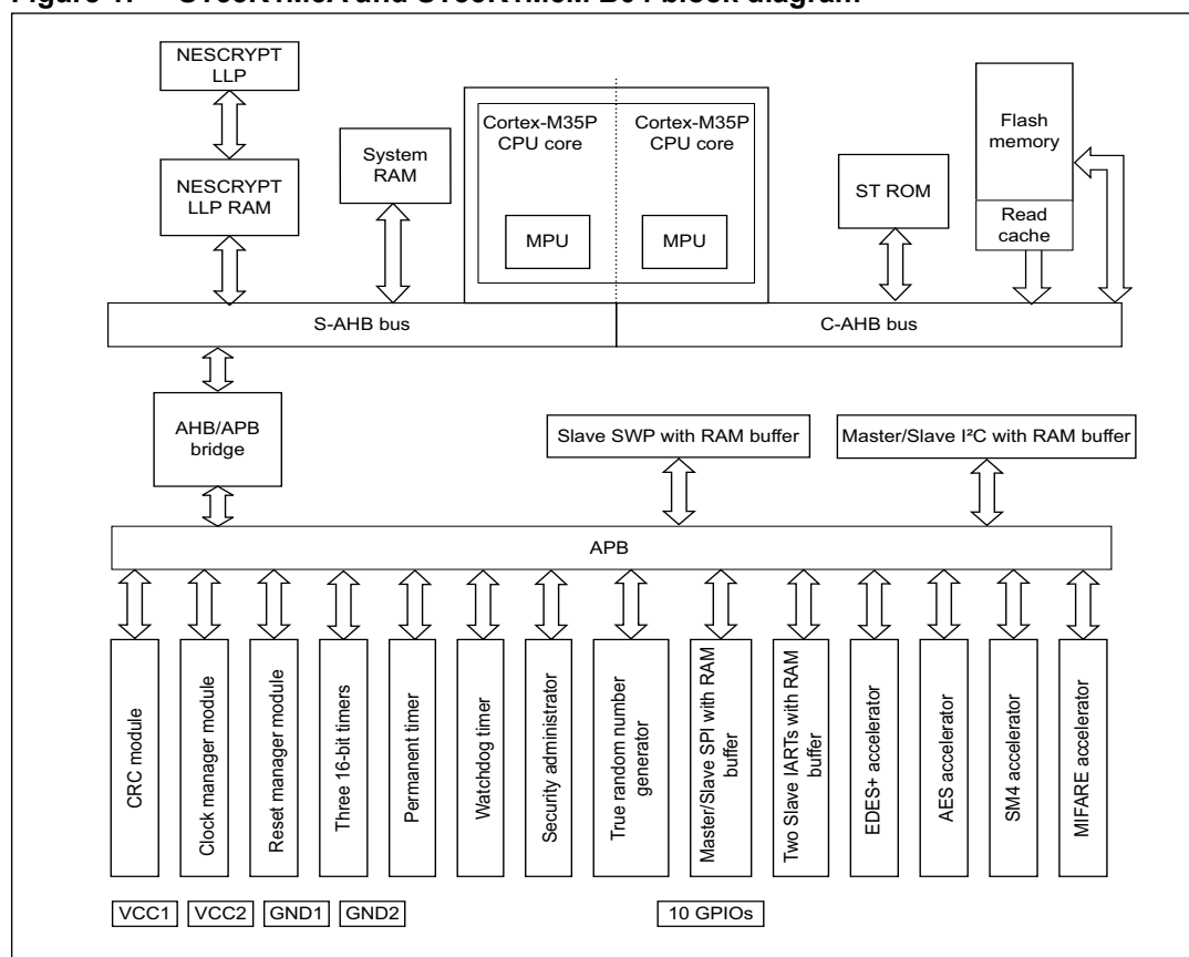
Figure 1. ST33K1M5A and ST33K1M5M B04 block diagram
