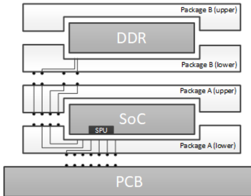
Figure 3-4 TOE package
