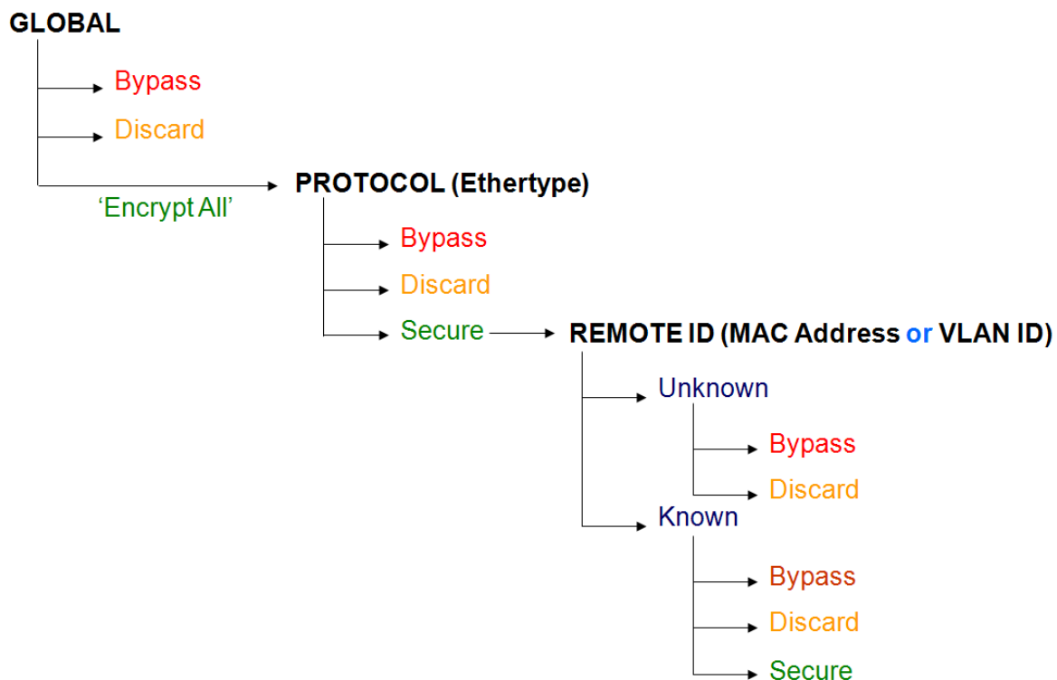
Figure 4 - Information Flow Control: Ethernet frame processing
