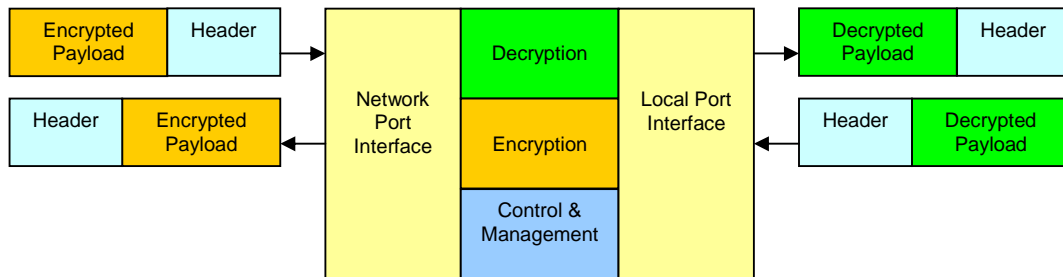
Figure 1 – Block Diagram
