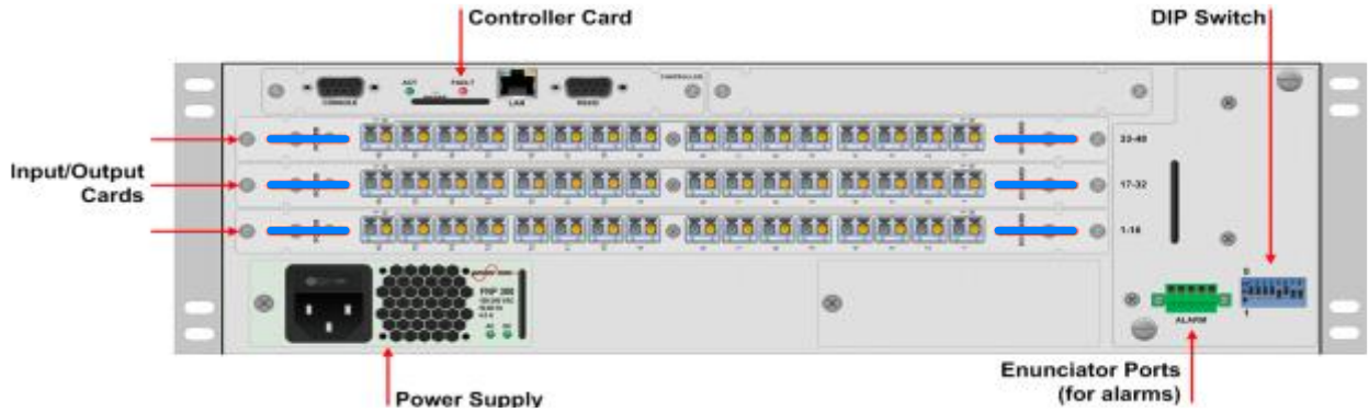
Figure 1a. Thinklogical TLX48 Matrix Switch
