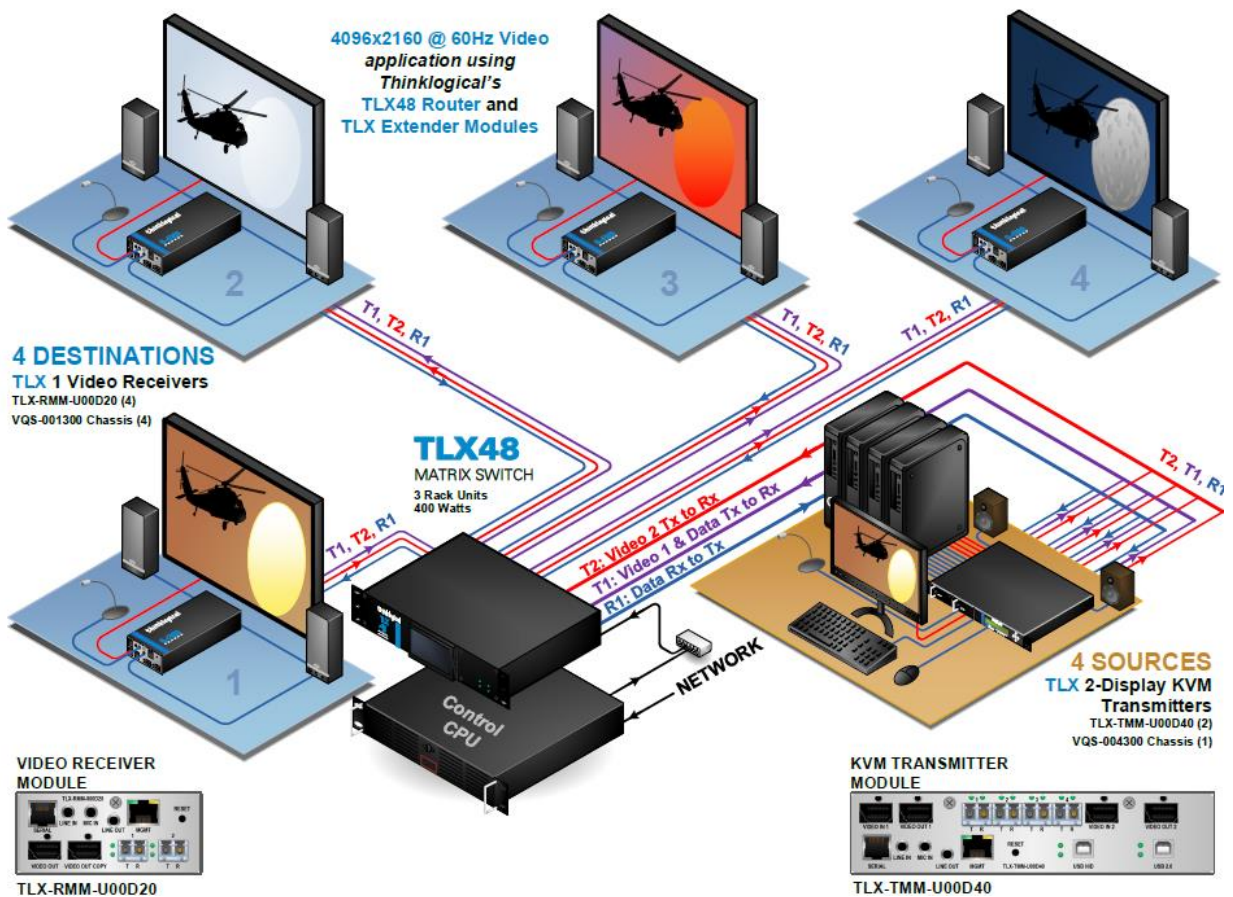
Figure 2a. Typical TOE TLX48 Matrix Switch (Front Mount Touch Panel)
