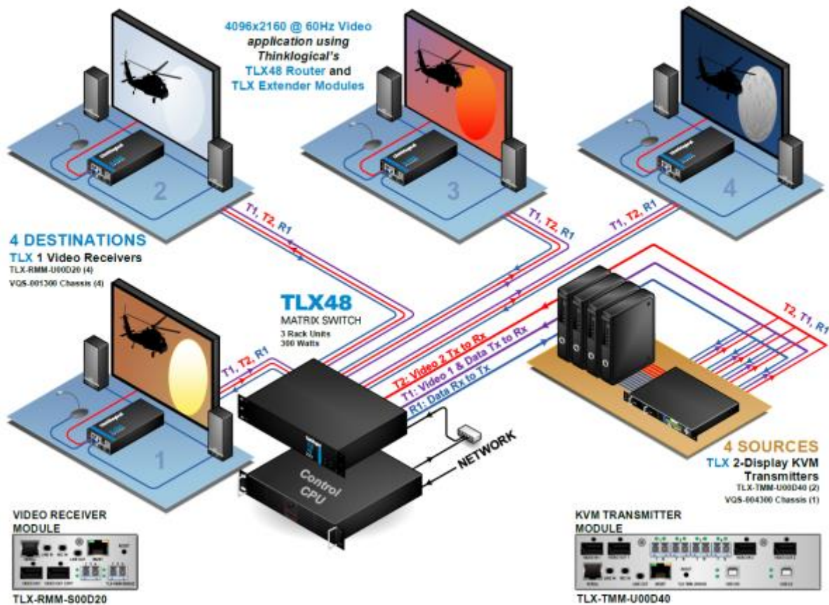
Figure 2b. Typical TOE TLX48 Matrix Switch (w/o Touch Panel)
