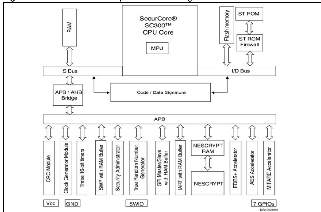
Figure 1. ST33G1M2AM C02 platform block diagram
