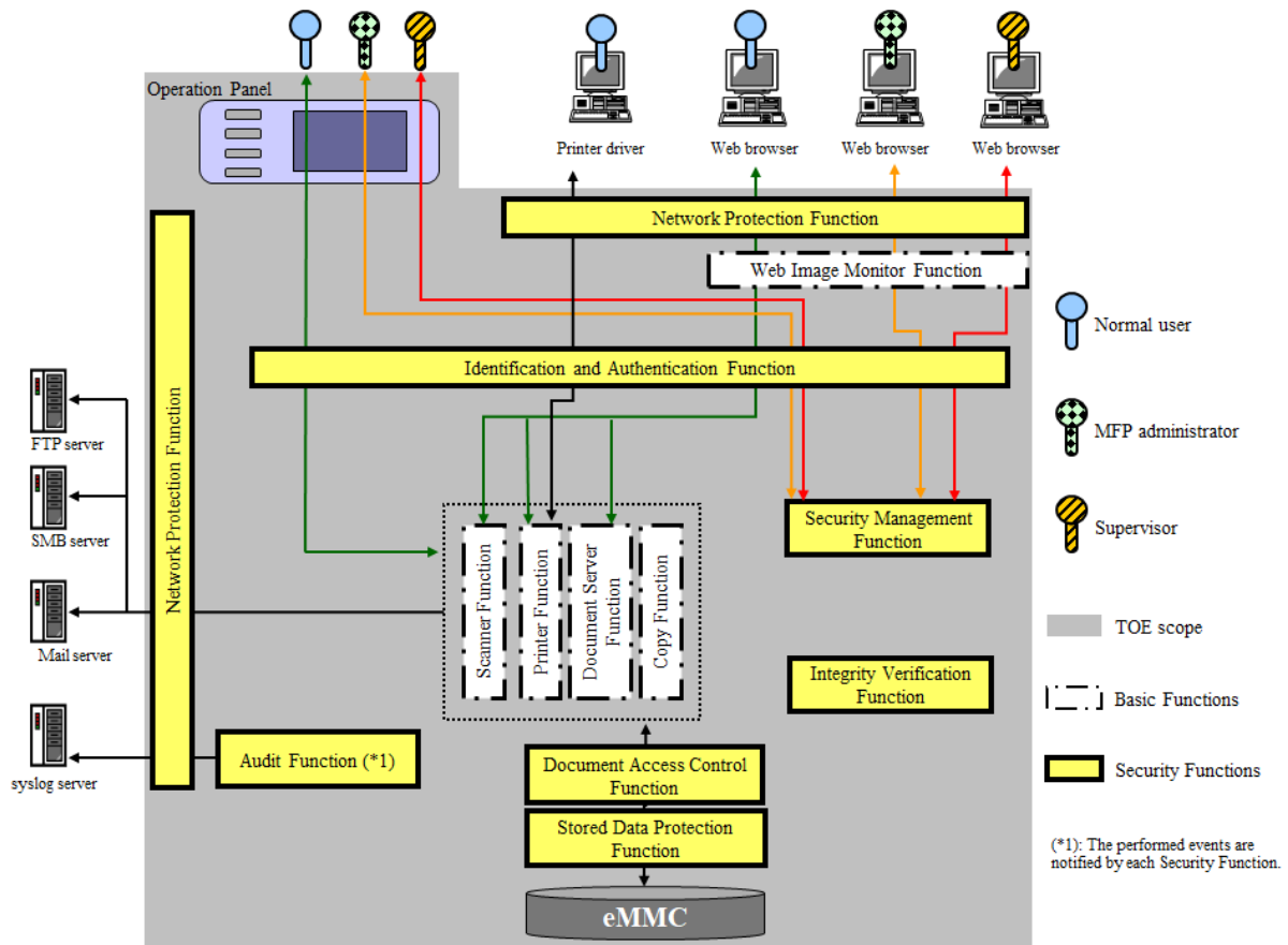
Figure 5-1 TOE Components
