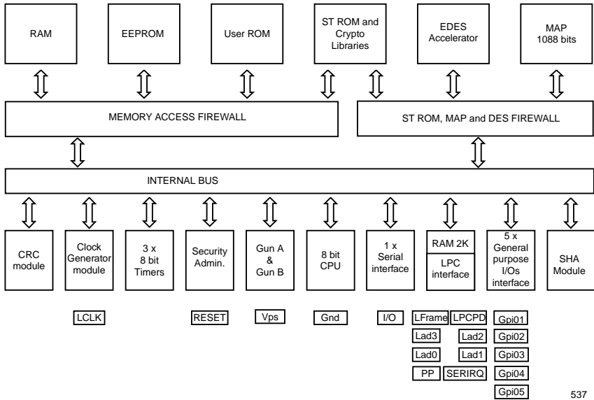
Figure 1 ST19WP18 block diagram
