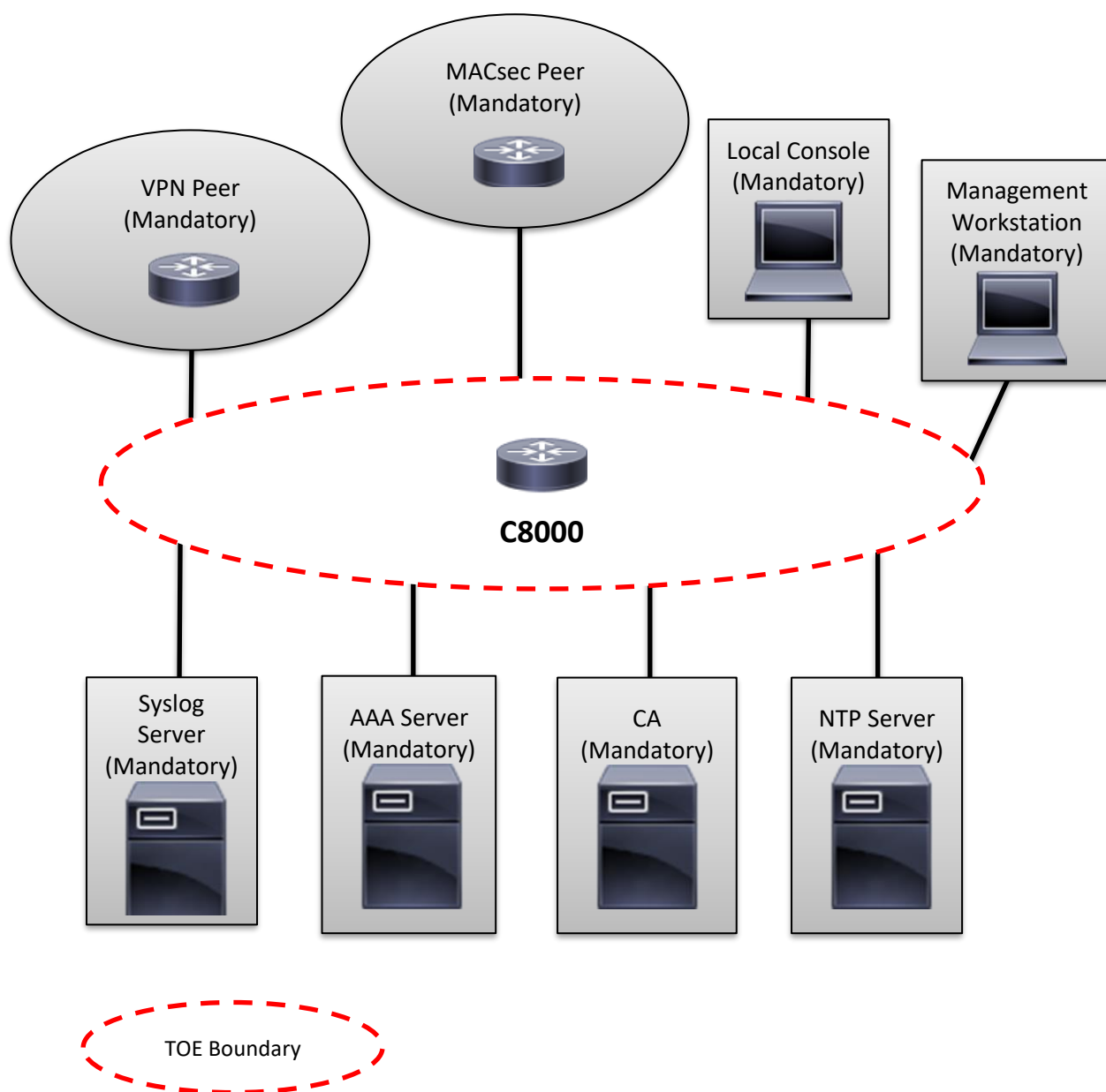
Figure 1 TOE Example Deployment for C8000
