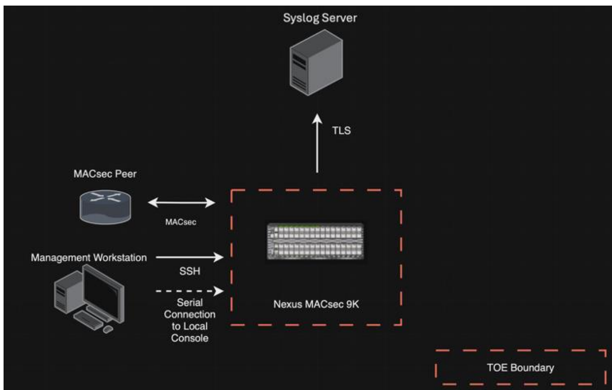
Figure 1 Nexus MACsec 9K TOE and Environment
